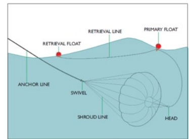
Key components of a para anchor deployment
